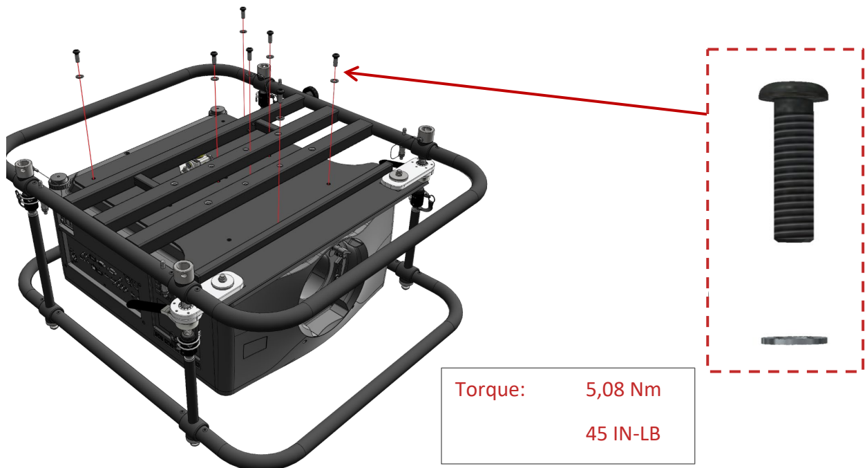
Figure 6 Securely tighten all screws
