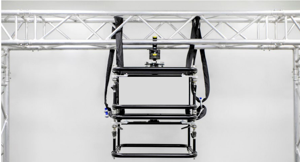
Figure 24 Securing two frames with two sets of rigging slings
