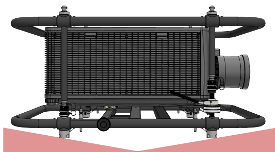
Figure 18 Adjustment: Pitch
