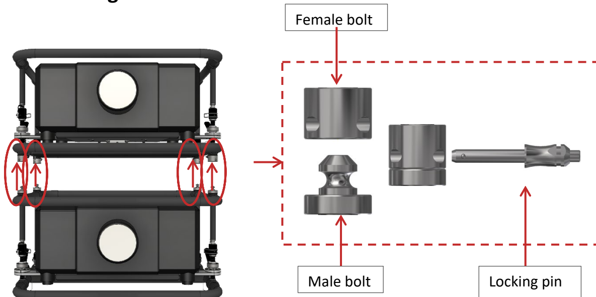
Figure 20 Stacking frames
