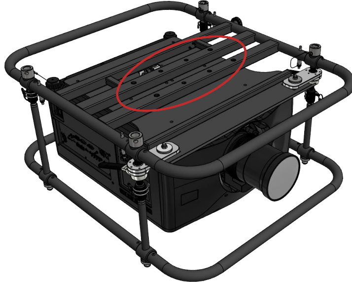
Figure 21 Threaded holes on bottom side of frame
