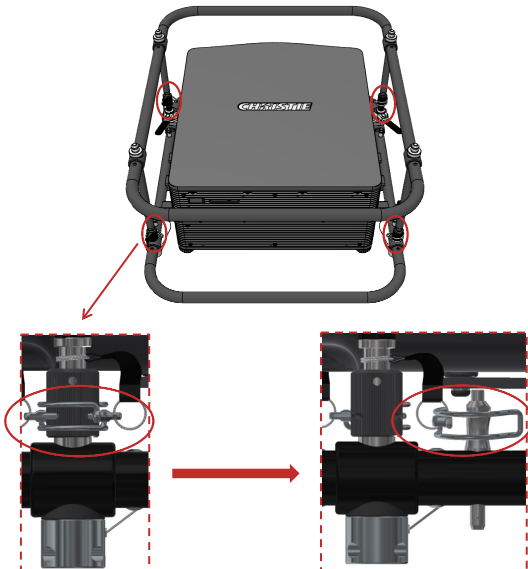
Figure 10 Removing the four spring clips
