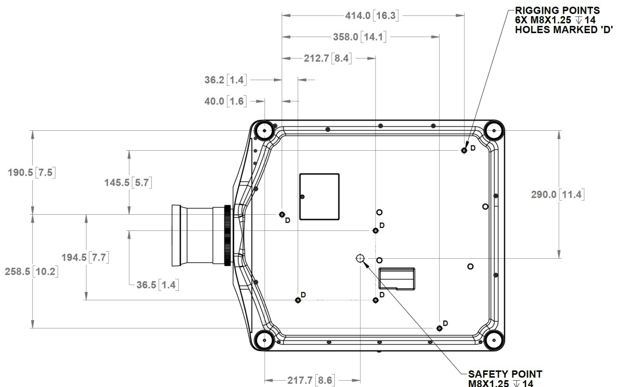
Figure 9 Drawing Bottom Side by Christie
