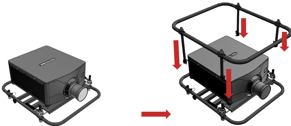
Figure 13 Reposition the upper ring
