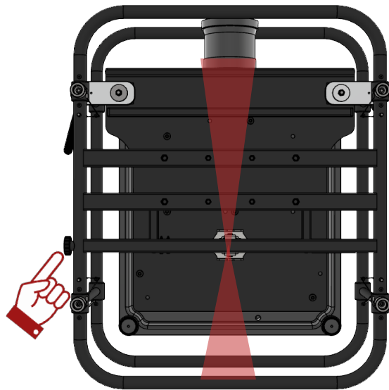
Figure 19 Adjustment: Yaw
