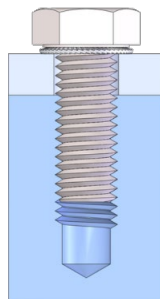
Figure 8 Schnorr safety washer correct orientation (Picture by Schnorr)
