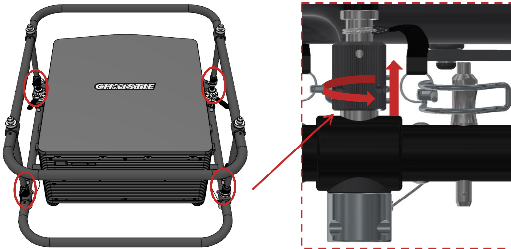
Figure 11 Unscrew the four attachment nuts
