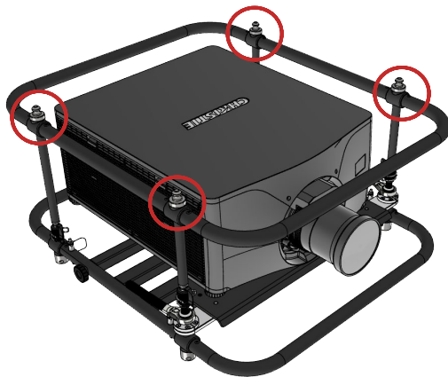
Figure 28 Stacking points topside
