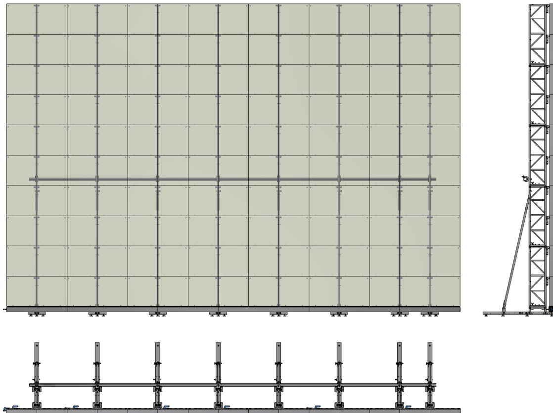
Figure 36 DB Series 15x10 Views
