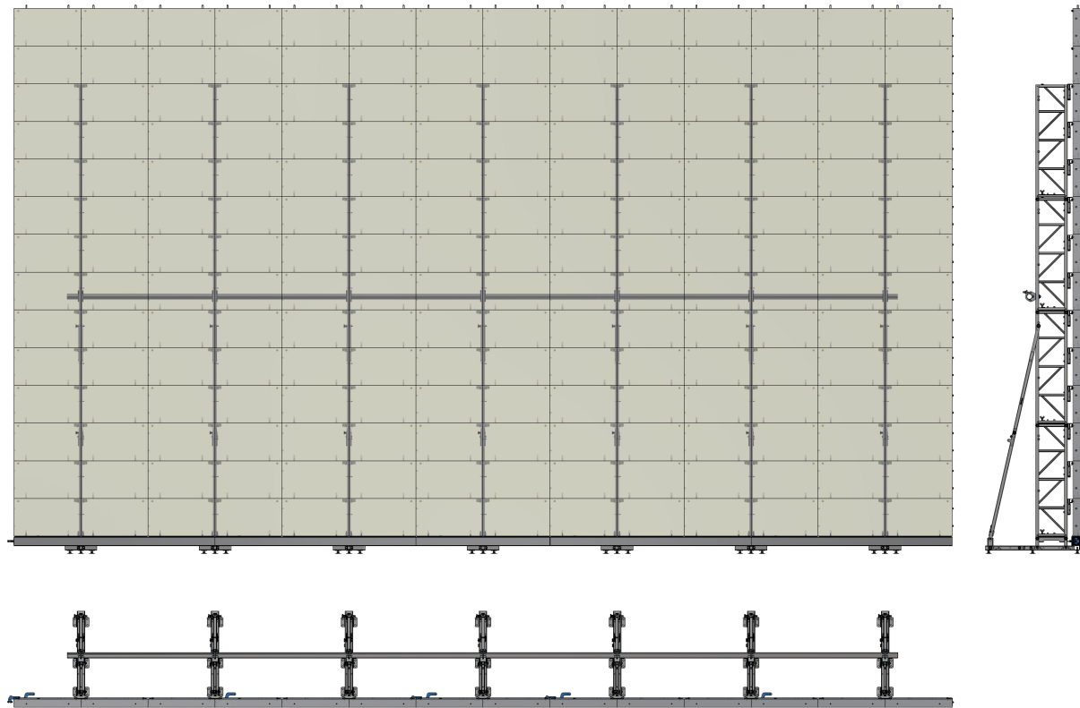
Figure 38 Absen AXpro 14x14 Views
