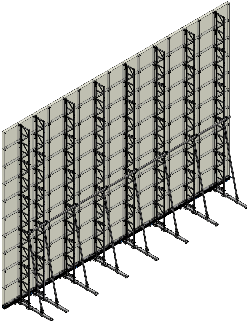
Figure 35 DB Series 15x10 Isometric View
