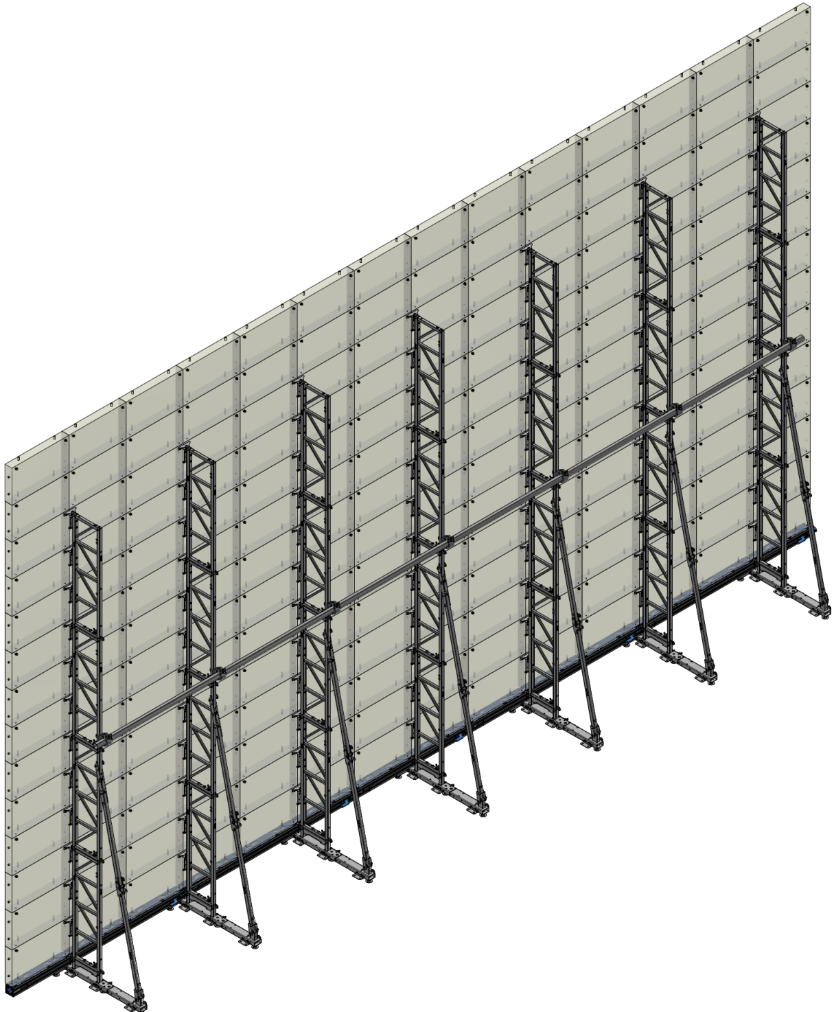
Figure 37 Absen AXpro 14x14 isometric view
