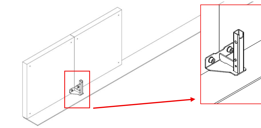
Figure 36 Montage der NoBase Clamps
