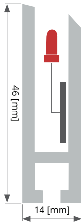
cross section primeTOUCH profile
