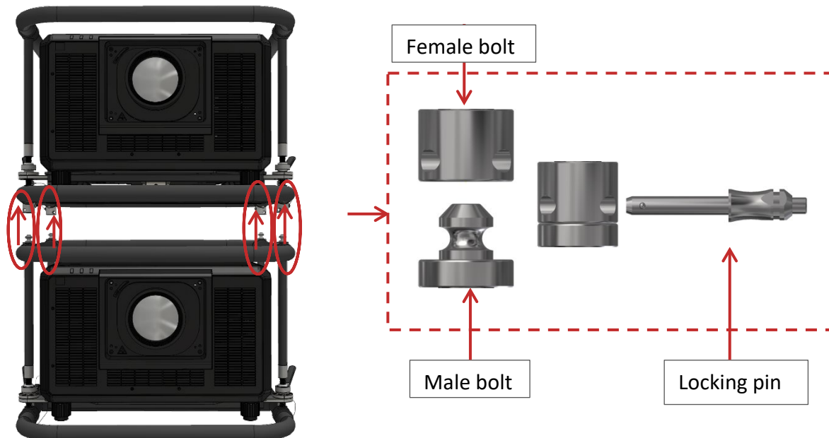
Figure 12 Stacking frames
