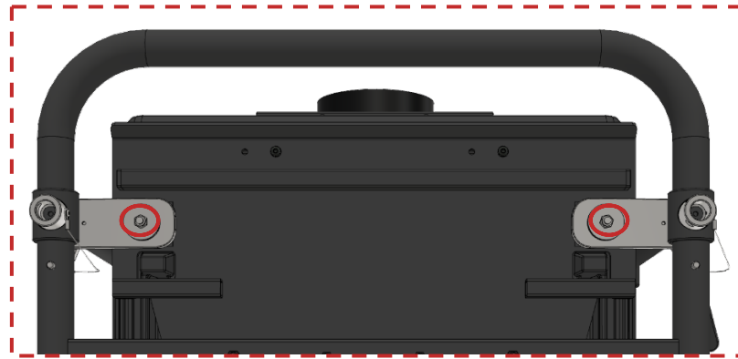
Figure 18 Nuts on front bottom side which are sealed with red colour wax
