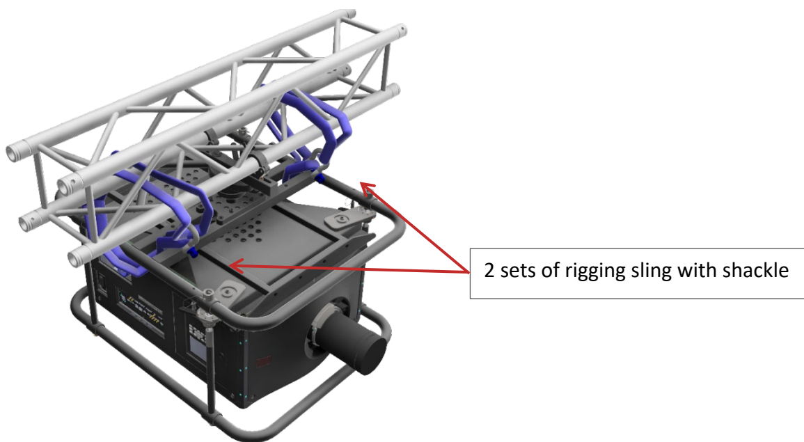
Figure 15 Securing one frame with two sets of rigging slings
