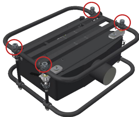
Figure 27 Stacking points bottom side
