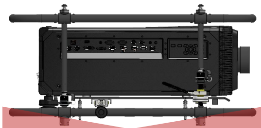
Figure 17 Adjustment: Pitch
