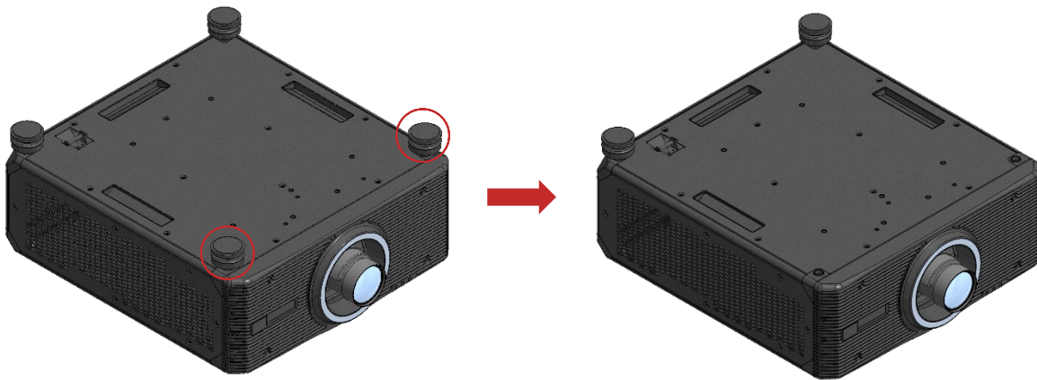
Figure 4 Removing the two front feet
