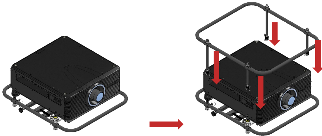
Figure 12 Reposition the upper ring
