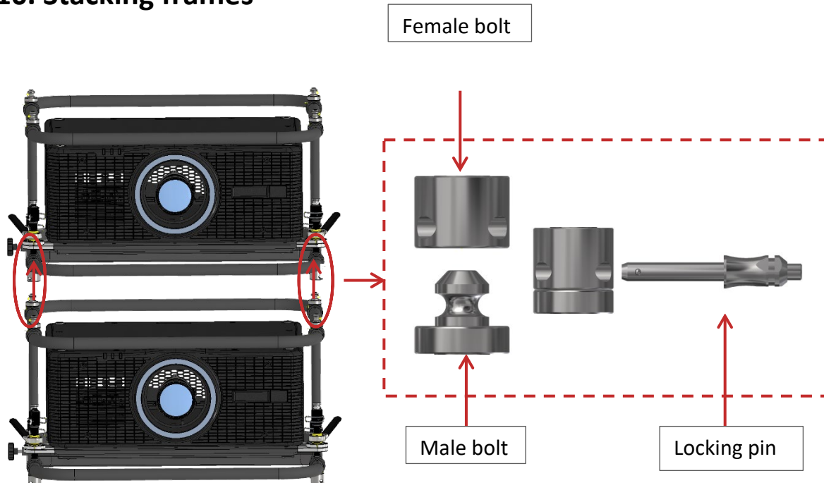
Figure 19 Stacking frames
