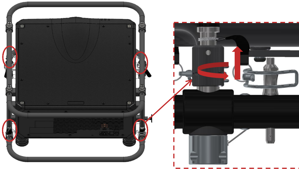
Figure 10 Unscrew the four attachment nuts
