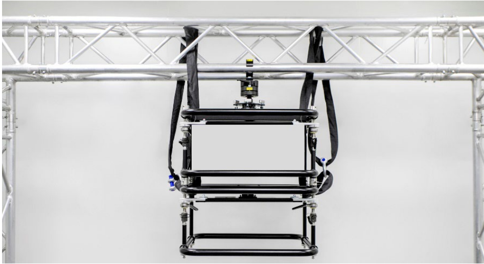
Figure 23 Securing two frames with two sets of rigging slings
