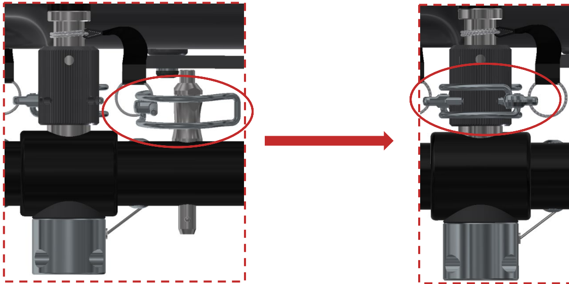
Figure 14 Reinsert the four spring clips and secure them
