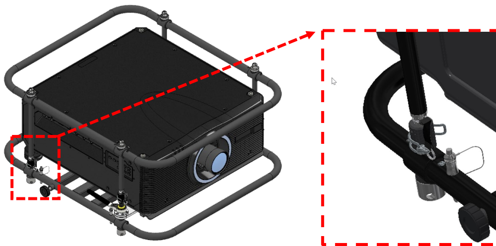
Figure 29 Locking pins at the frame
