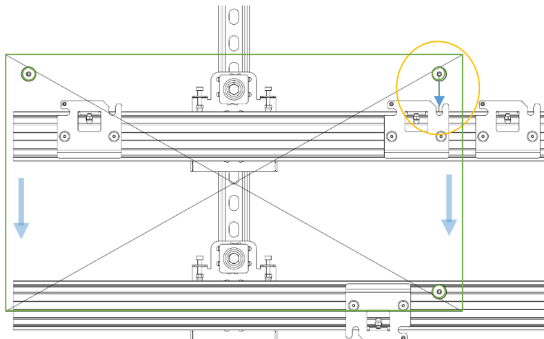
Figure 19 Cabinet moving towards keyhole
