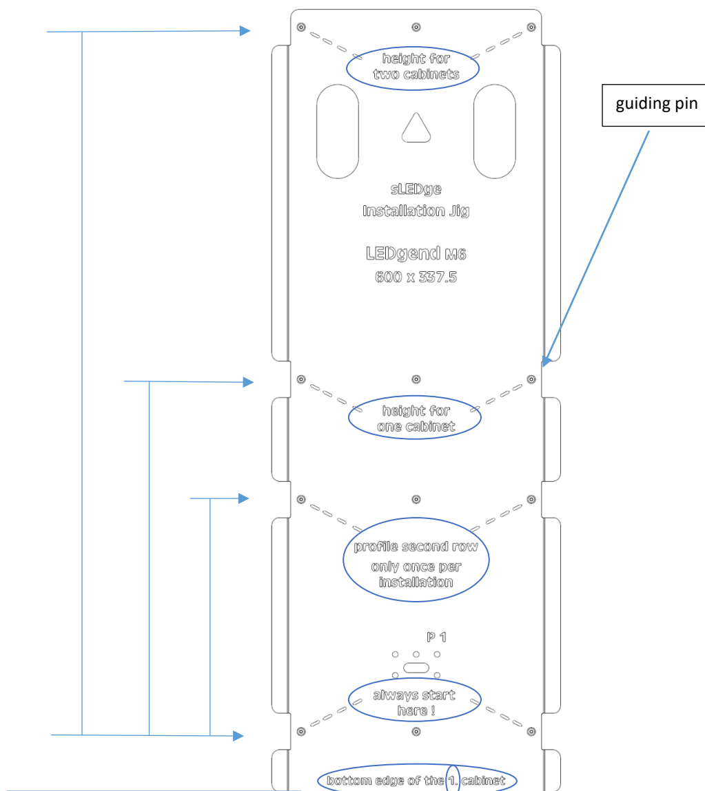
Figure 15 Exemplary illustration mounting jig
