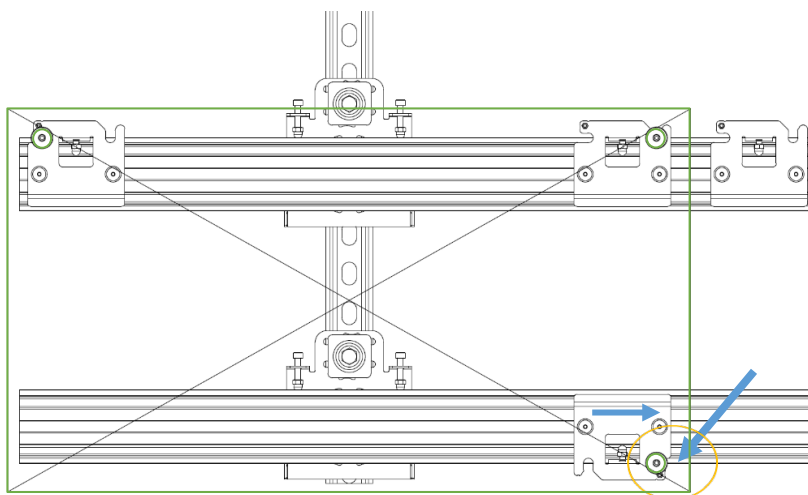
Figure 22 Keyhole lower right corner
