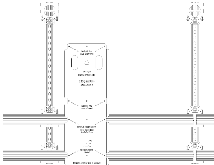
Figure 13 Front view jig in first and second row
