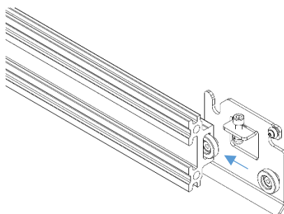
Figure 17 sliding the mounting plates into the profile (backside view)
