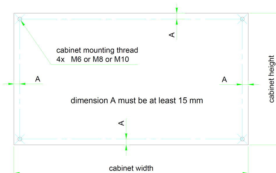
Figure 3 Rear view of a cabinet
