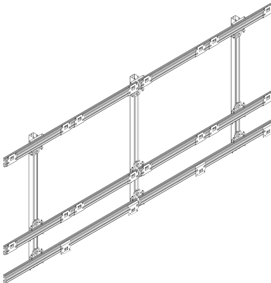
Figure 16 Exemplary overview for a 4x3 wall
