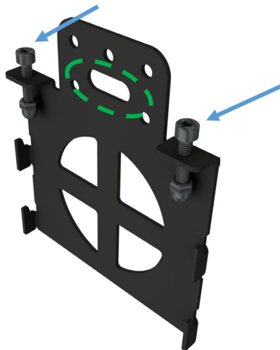
Figure 7 Fixation holes for C-Profile in wall mounting plate
