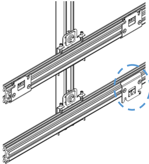
Figure 18 Lowest profile and rotated mounting plates
