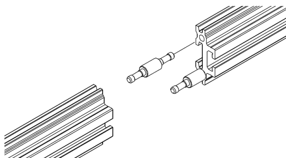
Figure 11 Profile connector
