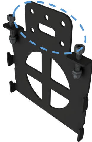
Figure 9 Fixation holes without C-Profile in wall mounting plate
