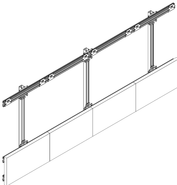
Figure 25 First cabinet row installed
