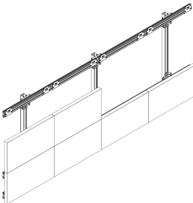
Figure 26 Second cabinet row partly installed
