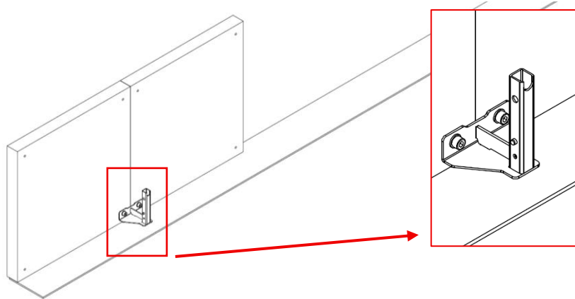
Figure 36 Mount NoBase Clamps
