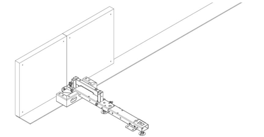
Figure 39 Attaching EXTENSION to SKI
