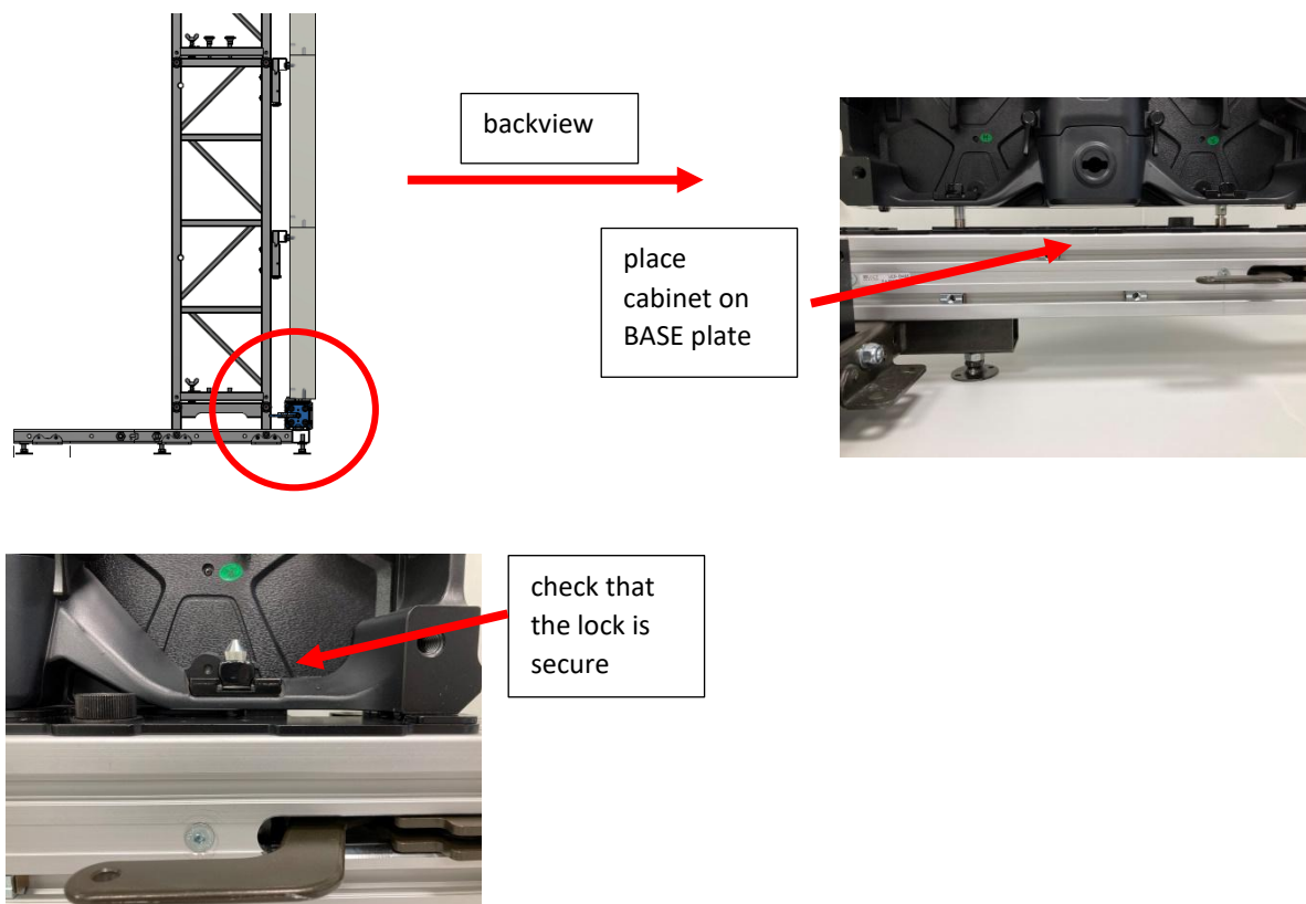
Figure 23 assembling LED cabinet (exemplary Infiled DB series)
