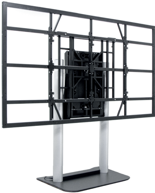
TITAN with mounting frame for LED unit (Landscape orientation)
