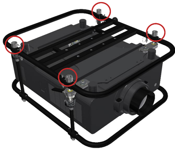
Figure 29 Stacking points bottom side
