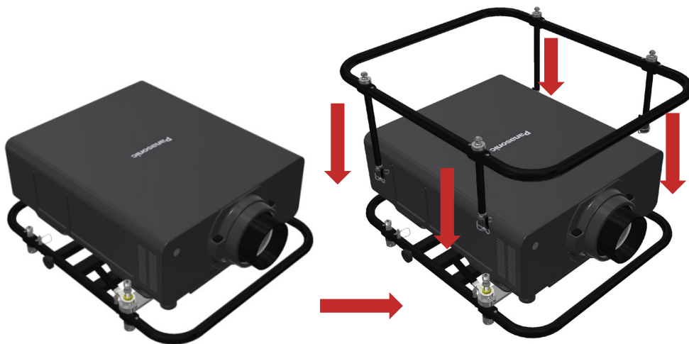
Figure 13 Reposition the upper ring
