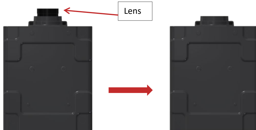
Figure 3 Removing the lens
