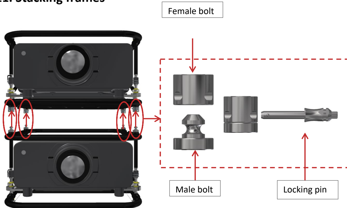
Figure 20 Stacking frames
