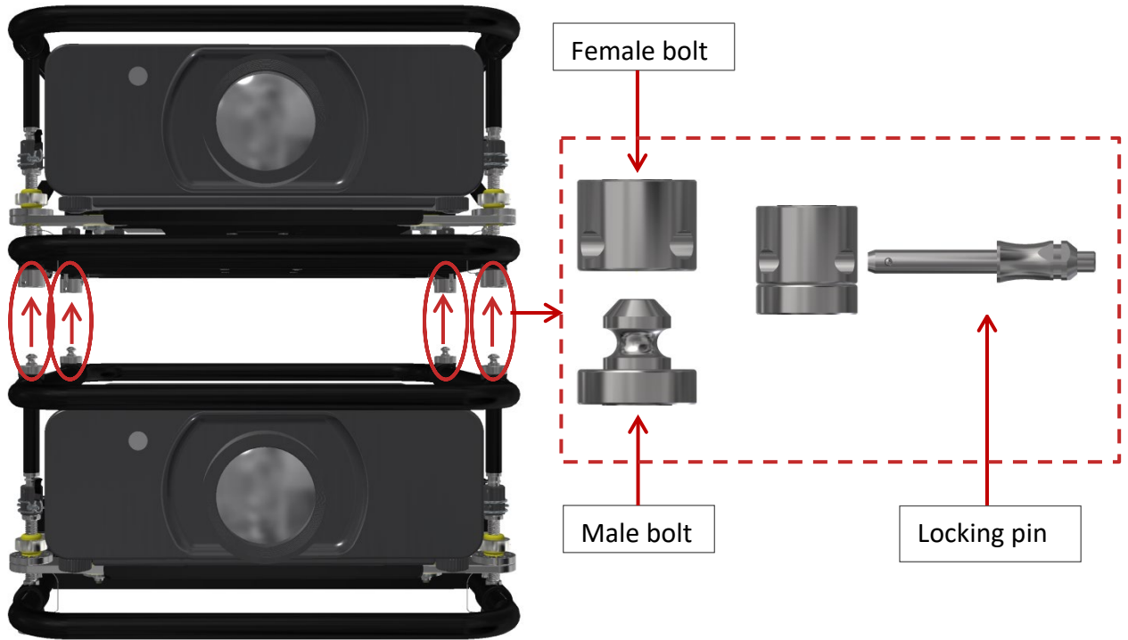
Figure 20 Stacking frames
