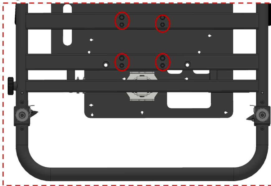
Figure 25 Inspection of mounting threads at bottom side
