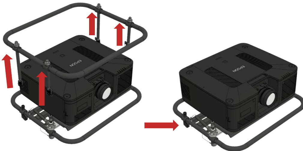
Figure 10 Remove the upper ring
