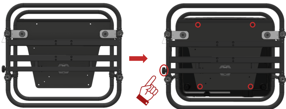
Figure 4 Mounting the projector into the frame
