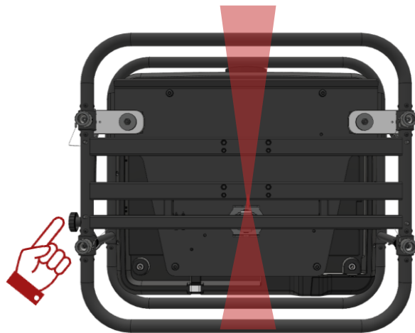
Figure 17 Adjustment: Yaw
