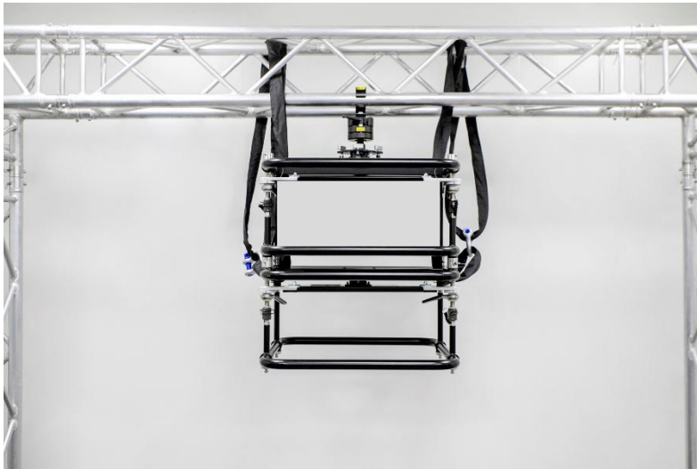
Figure 22 Securing two frames with two sets of rigging slings
