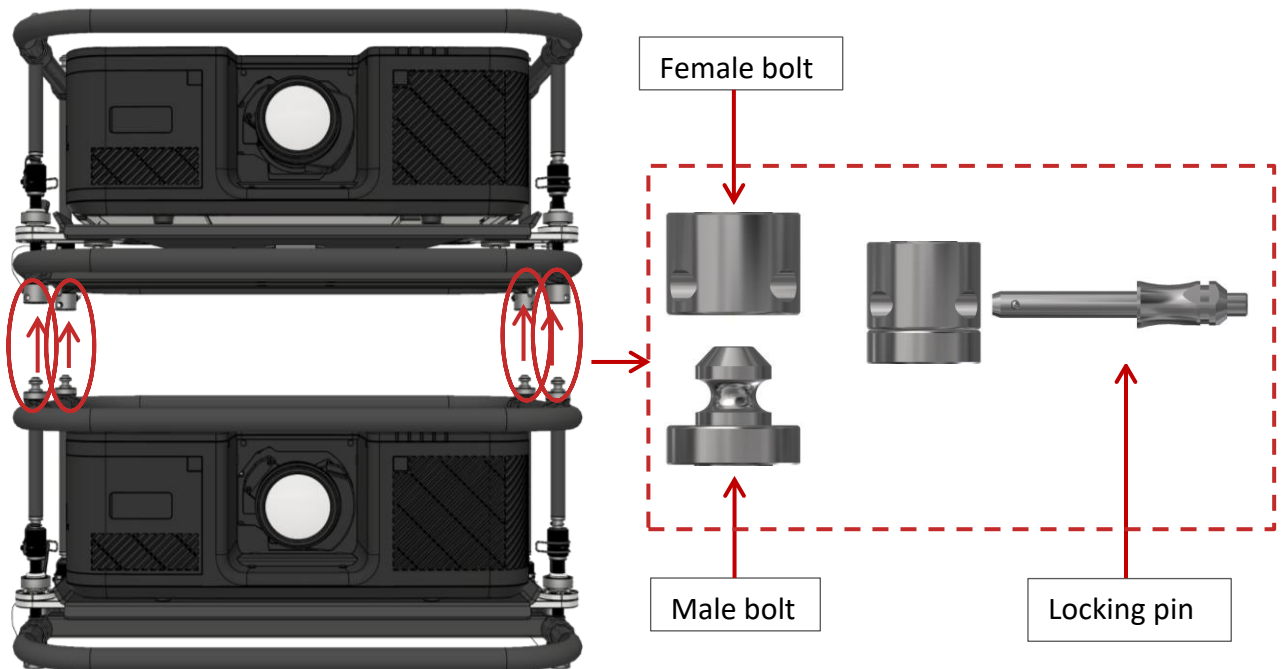
Figure 18 Stacking frames
