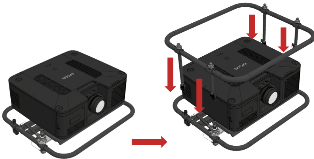
Figure 11 Reposition the upper ring
