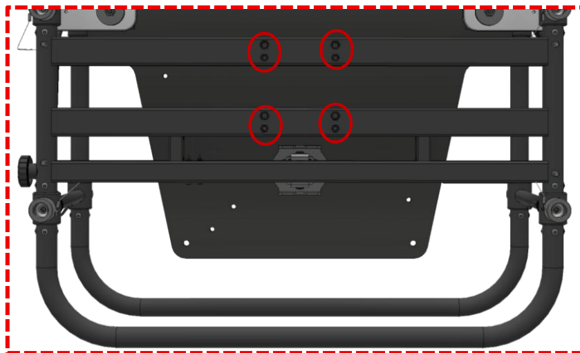
Figure 23 Inspection of mounting threads at bottom side
