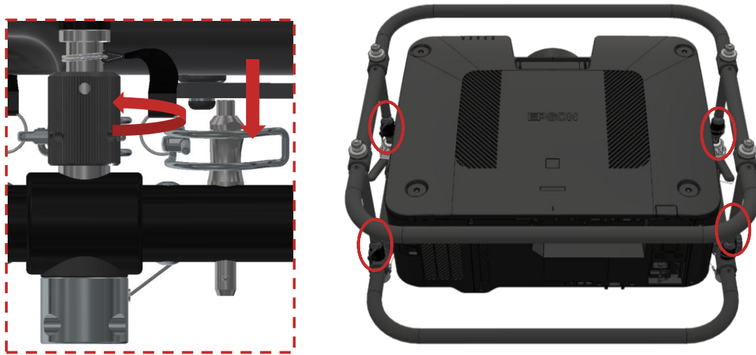
Figure 12 Tighten the four attachment nuts
