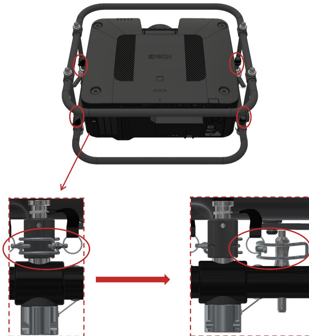
Figure 8 Removing the four spring clips
