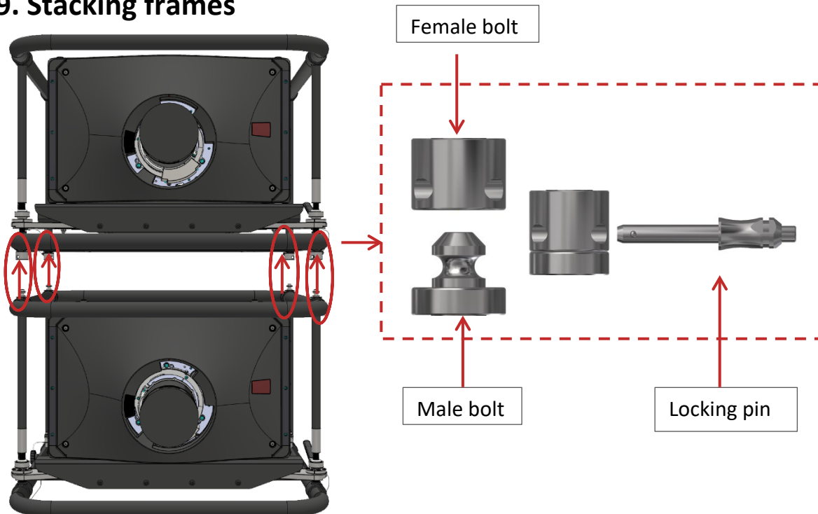
Figure 9 Stacking frames
