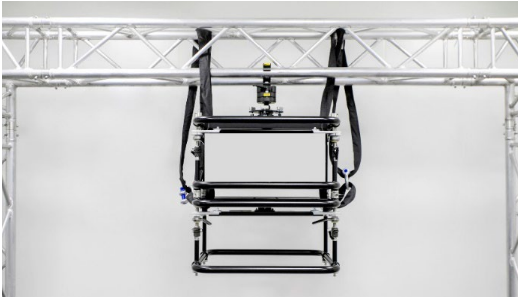
Figure 13 Securing two frames with two sets of rigging slings
