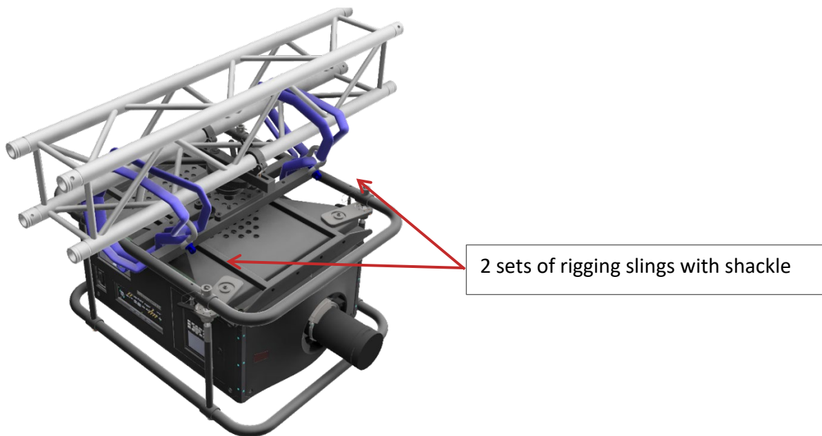
Figure 12 Securing one frame with two sets of rigging slings
