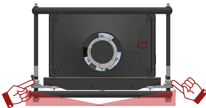
Figure 6 Adjustment: Roll
