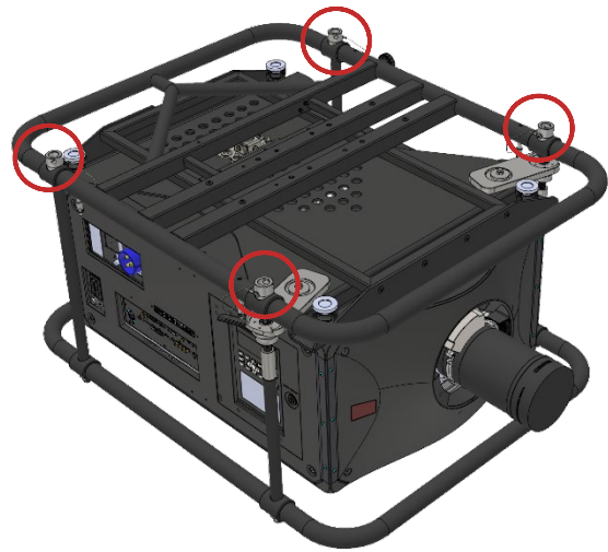
Figure 18 Stacking points bottom side
