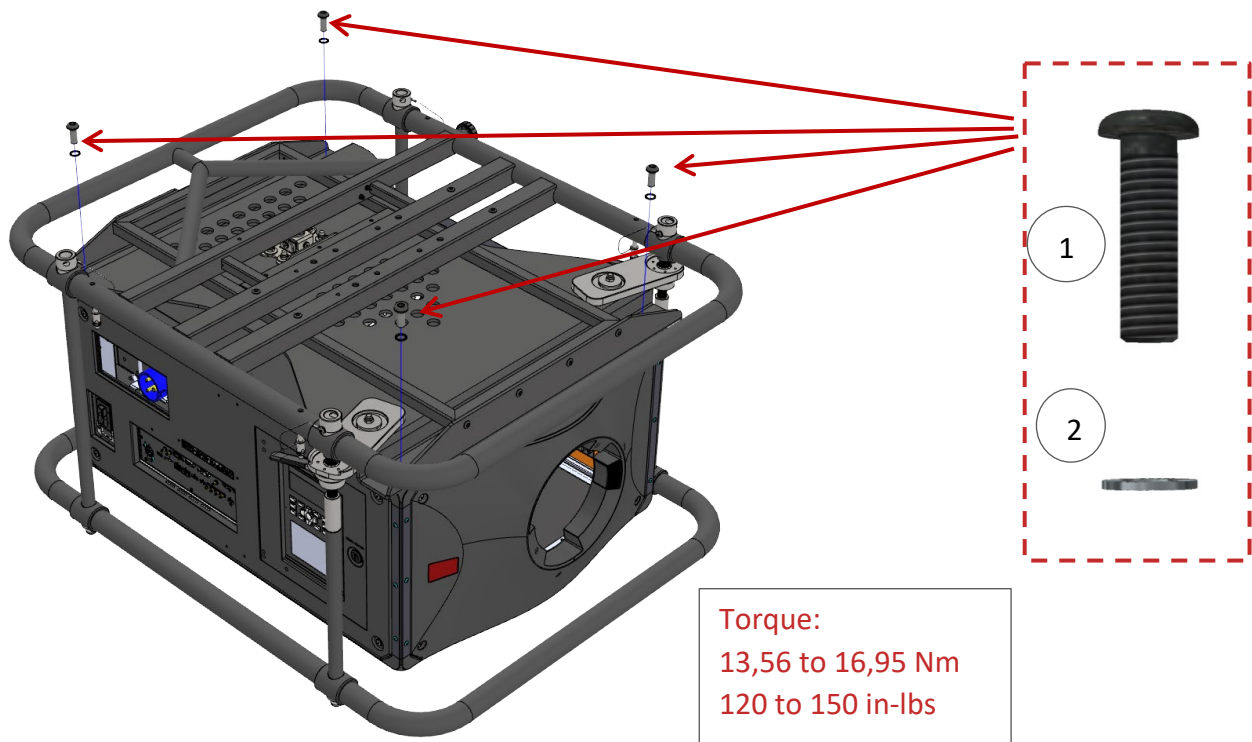
Figure 4 Securely tighten all screws
