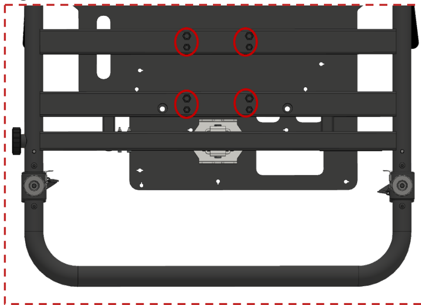
Figure 23 Inspection of mounting threads at bottom side
