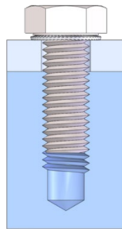
Figure 7 Schnorr safety washer correct orientation (Picture by Schnorr)
